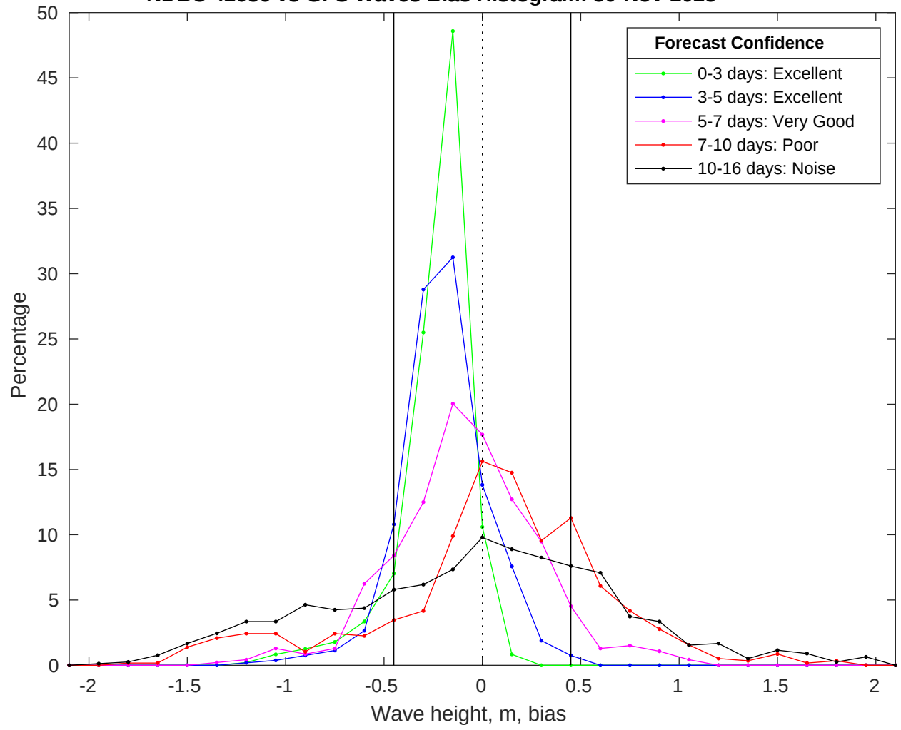
NDBC 42036 vs GFS Waves Bias Histogram: 30-Nov-2025
