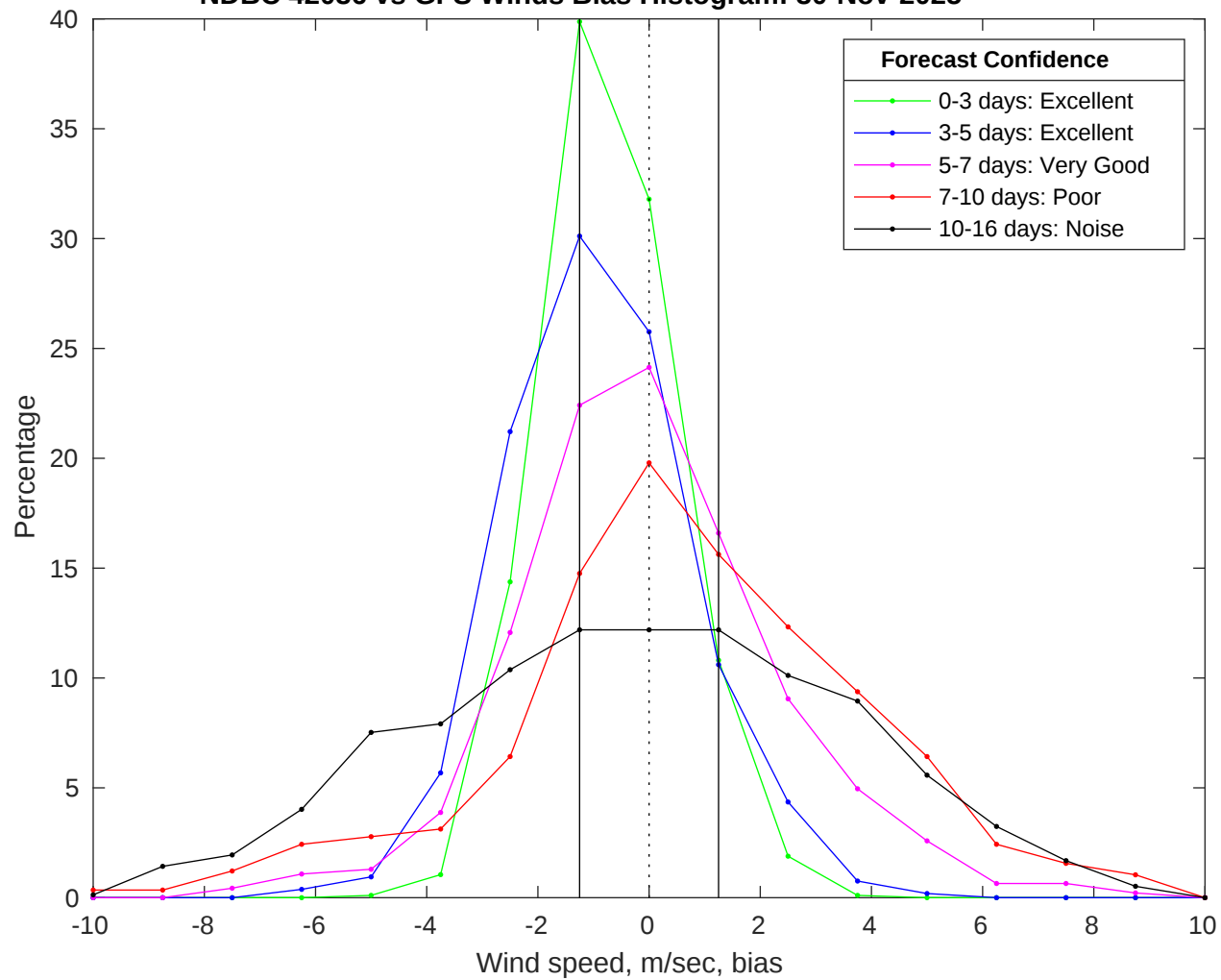
NDBC 42036 vs GFS Winds Bias Histogram: 30-Nov-2025
