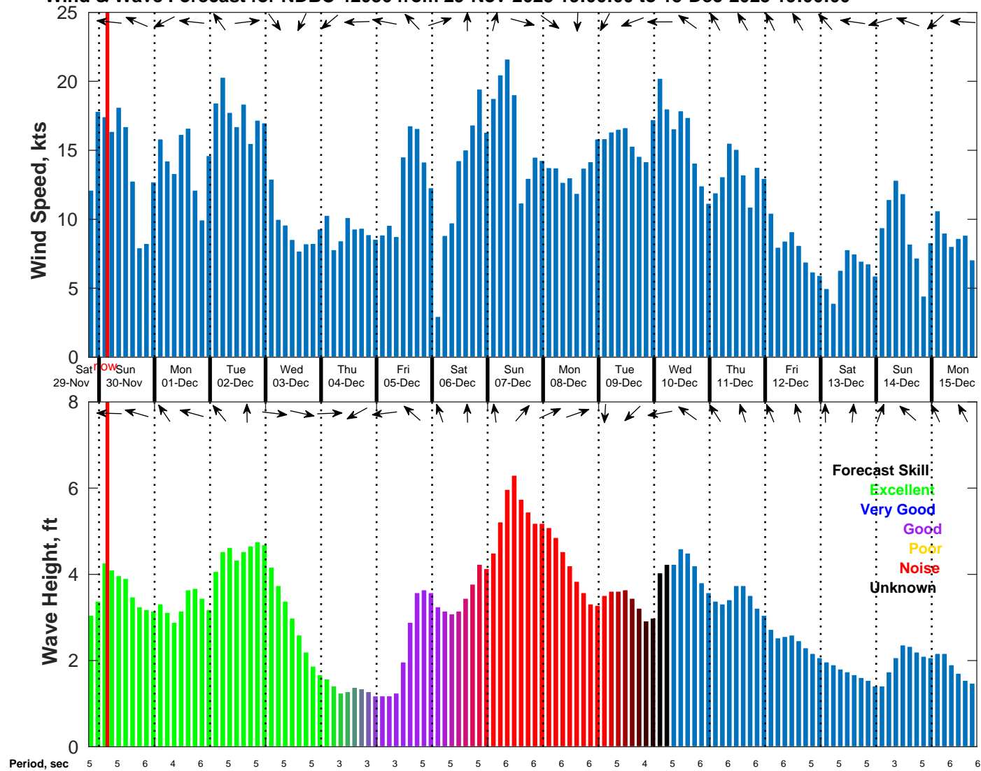
Wind & Wave Forecast for NDBC 42036 from 29-Nov-2025 19:00:00 to 15-Dec-2025 19:00:00
