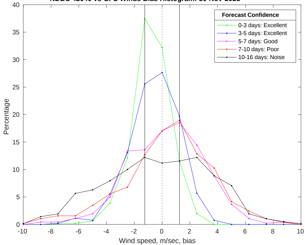
NDBC 42040 vs GFS Winds Bias Histogram: 30-Nov-2025
