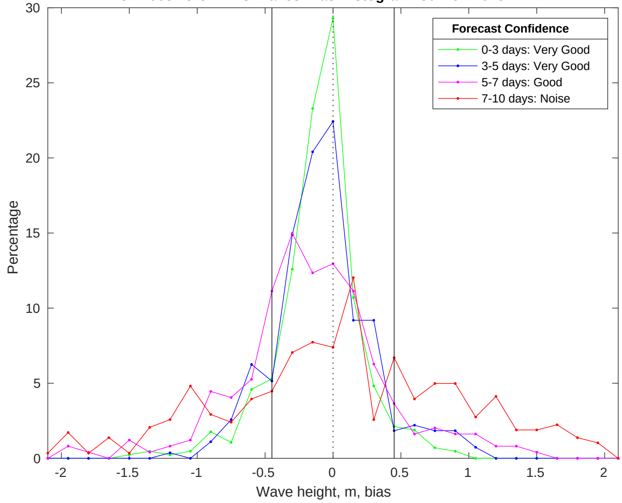
NDBC 44008 vs CMEMS Waves Bias Histogram: 30-Nov-2025
