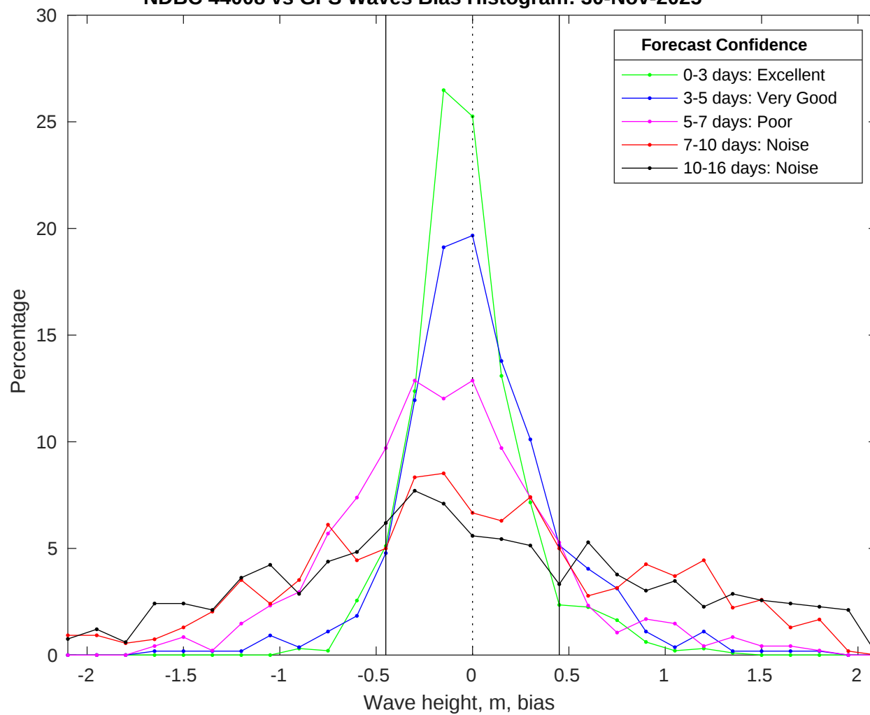
NDBC 44008 vs GFS Waves Bias Histogram: 30-Nov-2025
