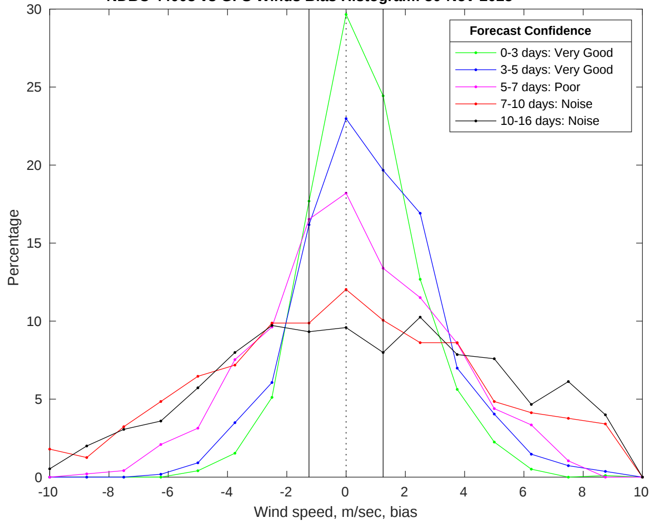
NDBC 44008 vs GFS Winds Bias Histogram: 30-Nov-2025
