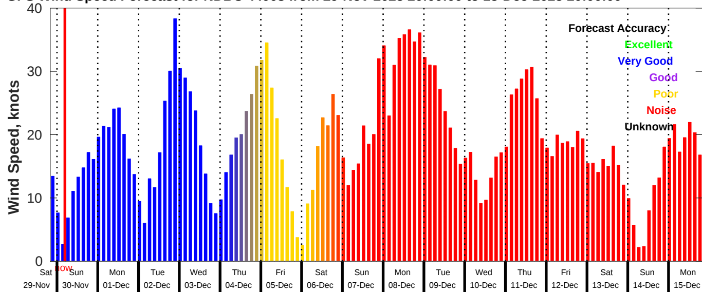
GFS Wind Speed Forecast for NDBC 44008 from 29-Nov-2025 20:00:00 to 15-Dec-2025 20:00:00
