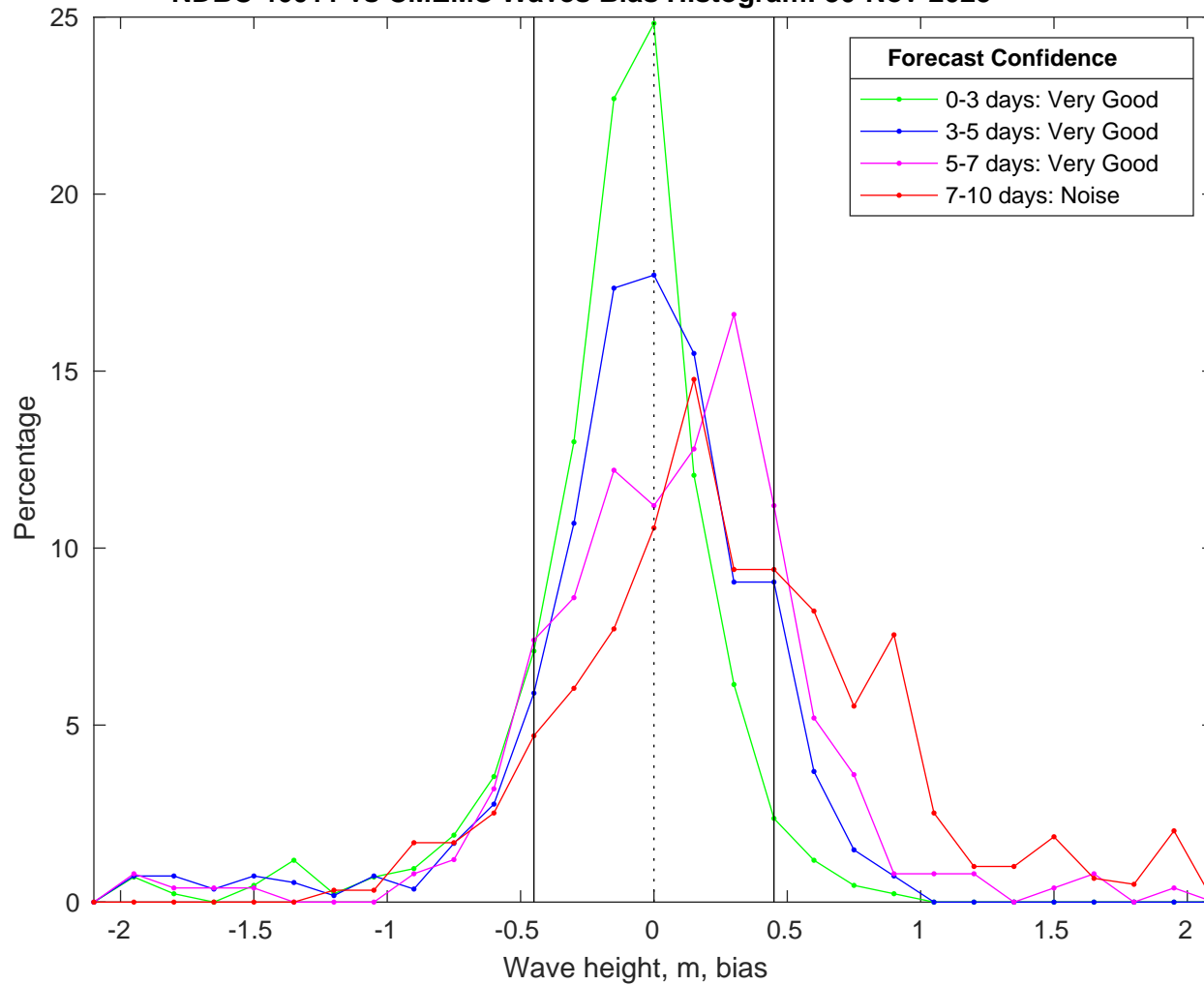
NDBC 46011 vs CMEMS Waves Bias Histogram: 30-Nov-2025
