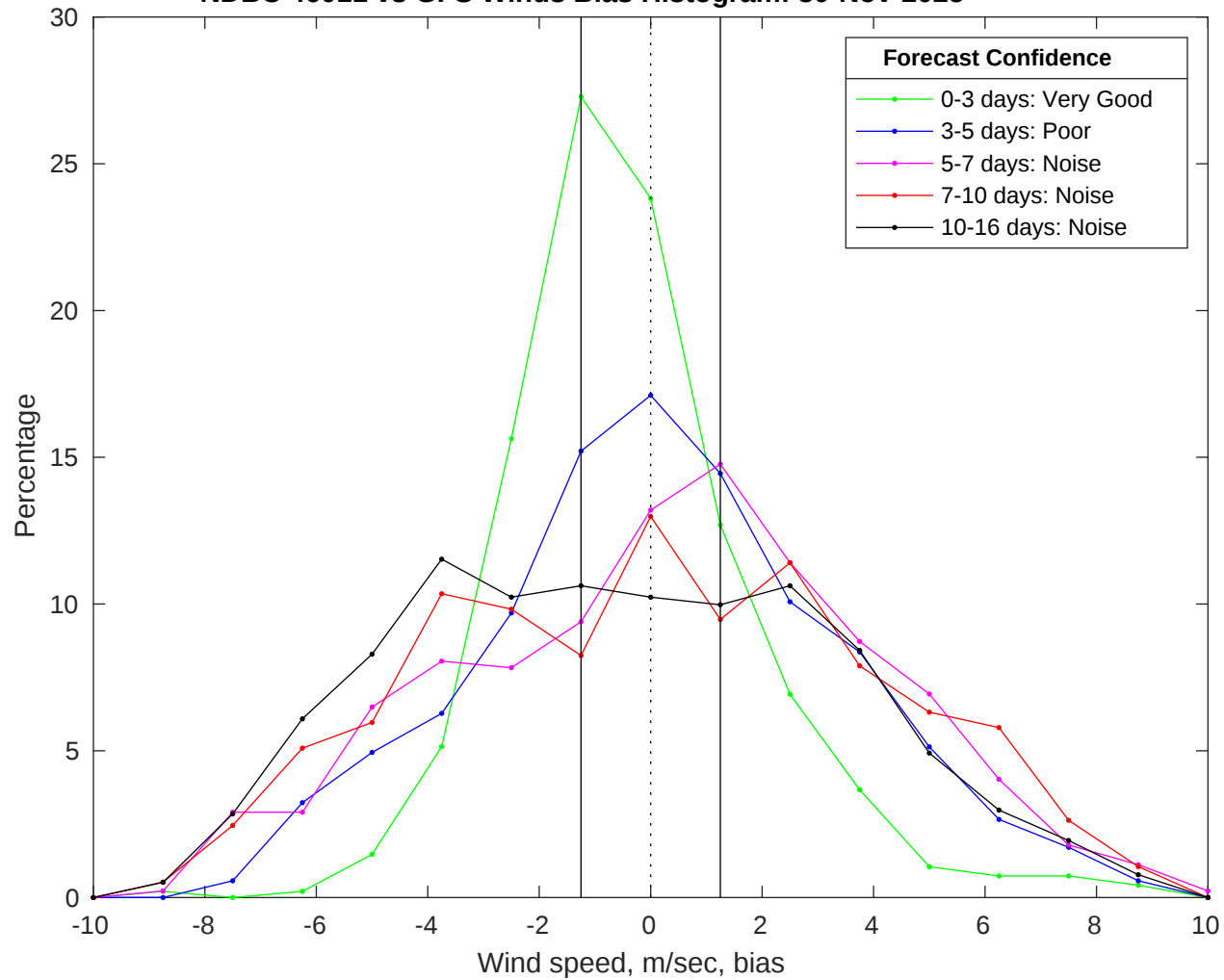
NDBC 46011 vs GFS Winds Bias Histogram: 30-Nov-2025
