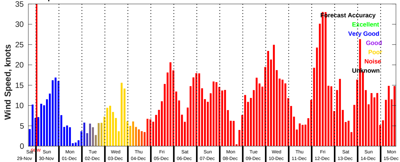
GFS Wind Speed Forecast for NDBC 46011 from 29-Nov-2025 16:00:00 to 15-Dec-2025 16:00:00
