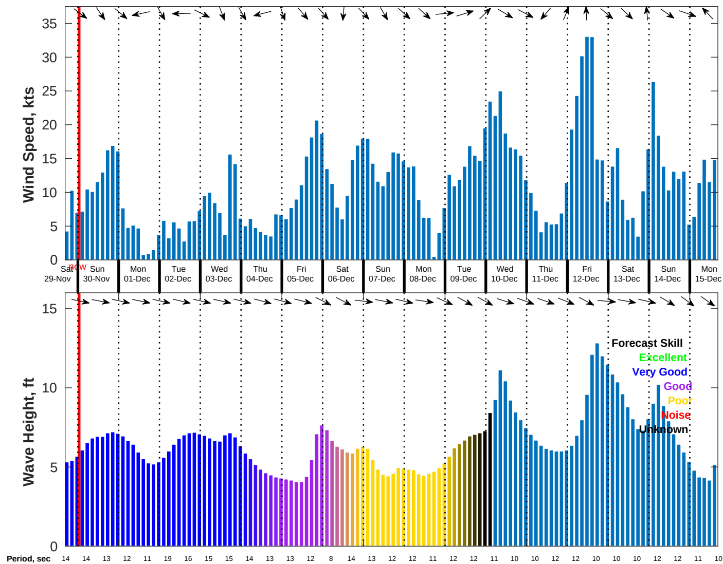
Wind & Wave Forecast for NDBC 46011 from 29-Nov-2025 16:00:00 to 15-Dec-2025 16:00:00
