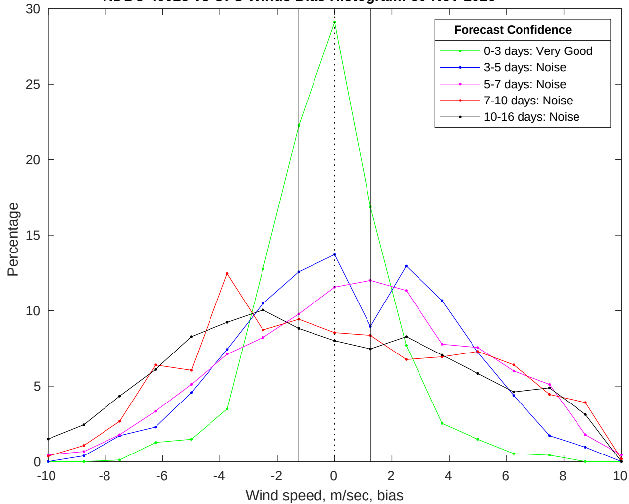
NDBC 46028 vs GFS Winds Bias Histogram: 30-Nov-2025
