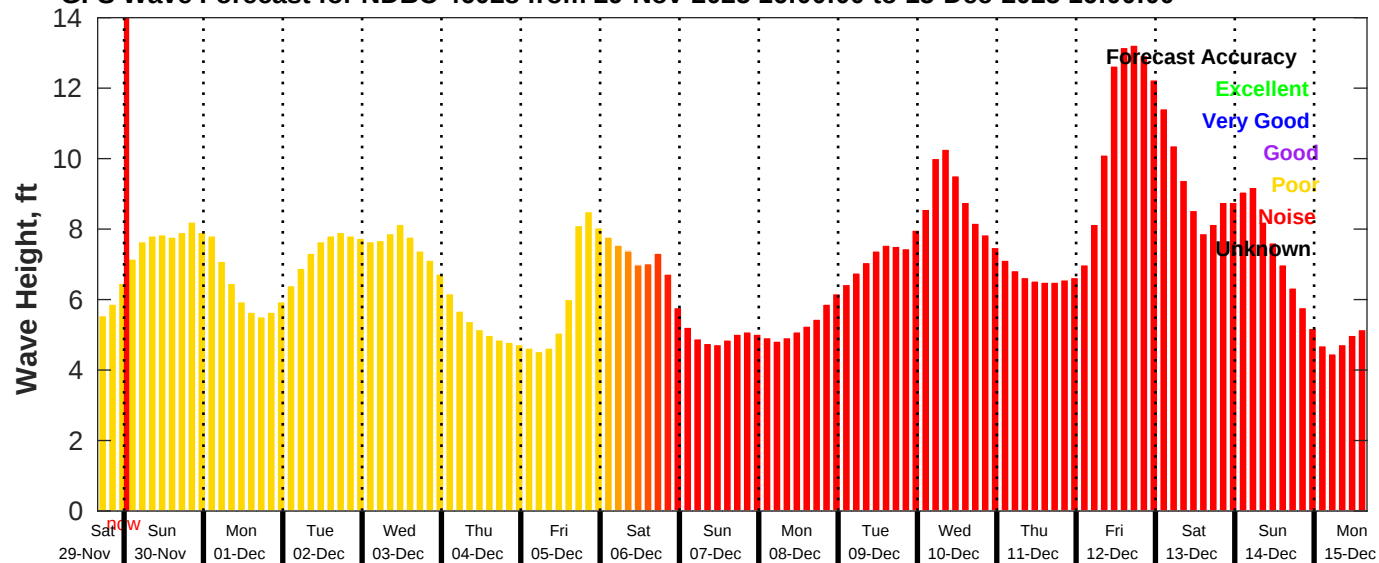
GFS Wave Forecast for NDBC 46028 from 29-Nov-2025 16:00:00 to 15-Dec-2025 16:00:00
