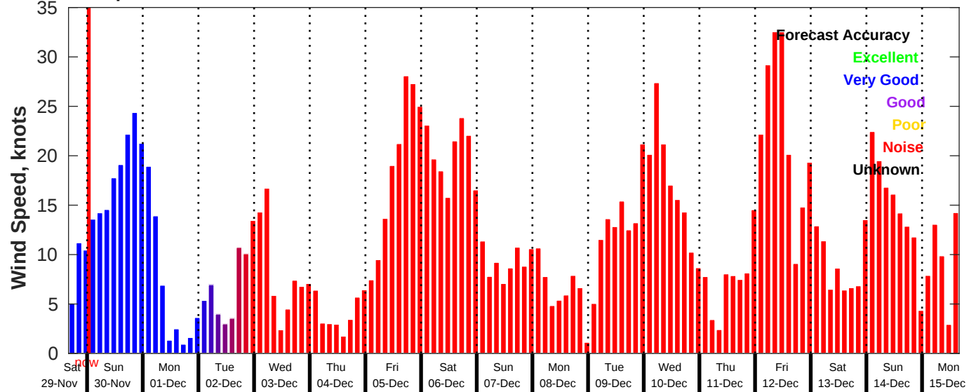
GFS Wind Speed Forecast for NDBC 46028 from 29-Nov-2025 16:00:00 to 15-Dec-2025 16:00:00
