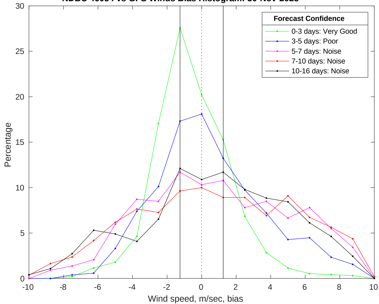
NDBC 46054 vs GFS Winds Bias Histogram: 30-Nov-2025
