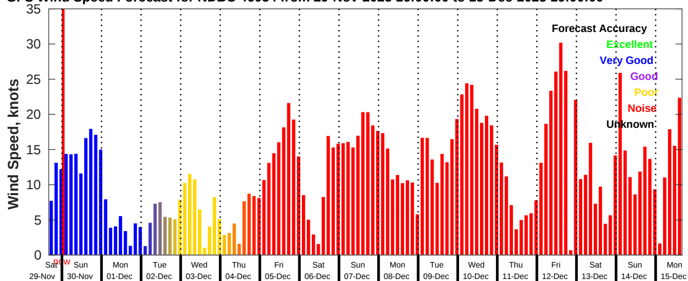
GFS Wind Speed Forecast for NDBC 46054 from 29-Nov-2025 16:00:00 to 15-Dec-2025 16:00:00
