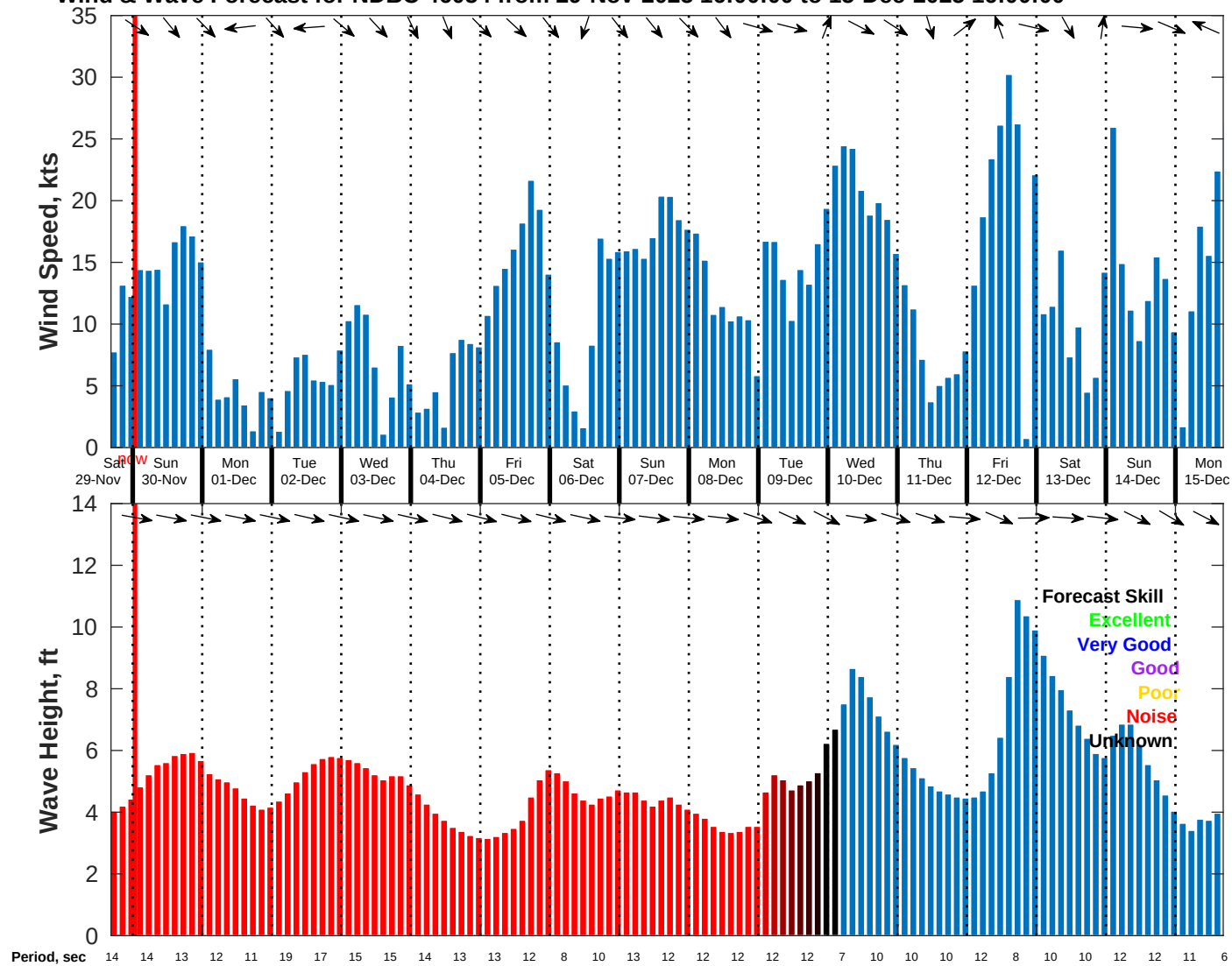
Wind & Wave Forecast for NDBC 46054 from 29-Nov-2025 16:00:00 to 15-Dec-2025 16:00:00
