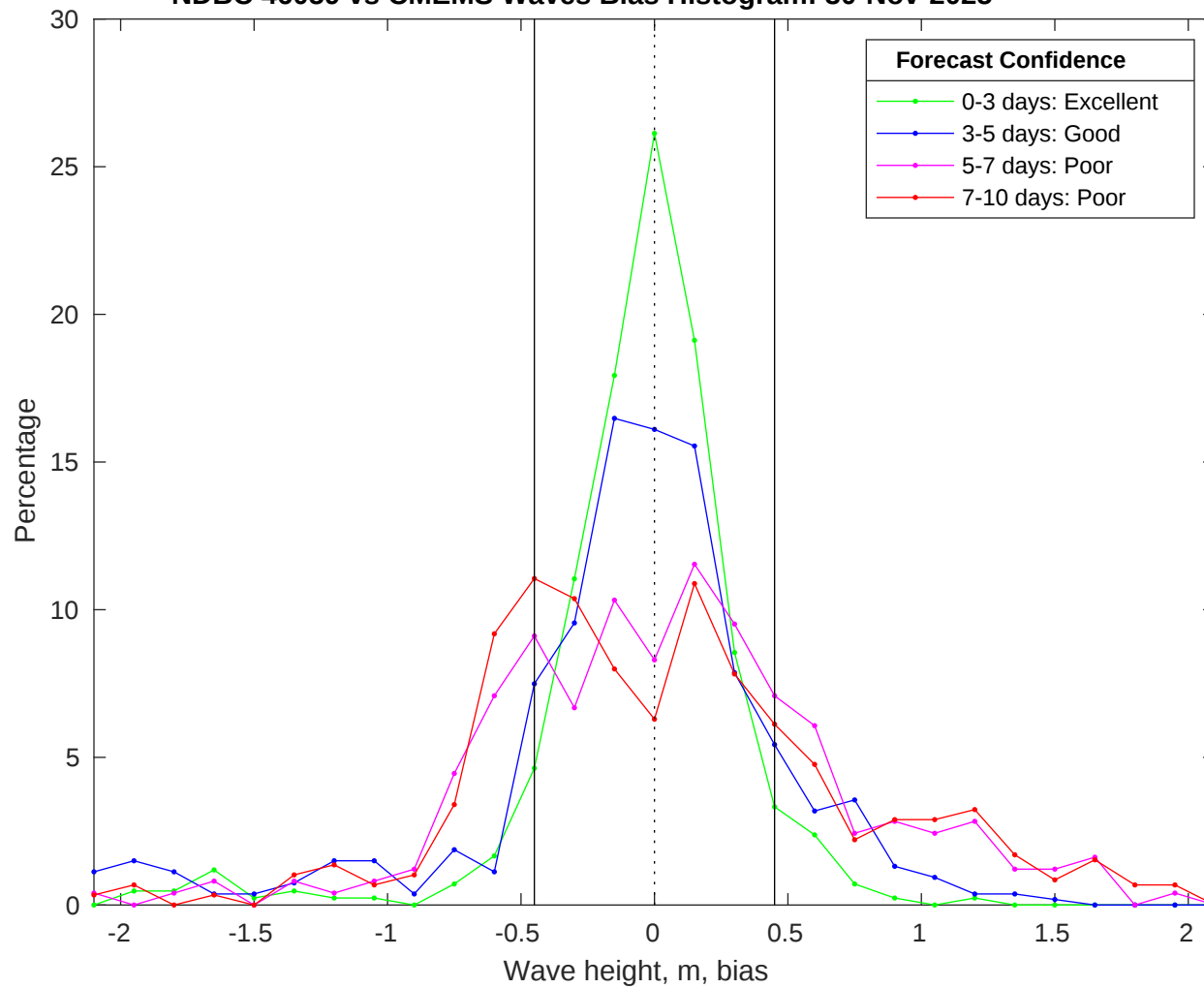
NDBC 46059 vs CMEMS Waves Bias Histogram: 30-Nov-2025
