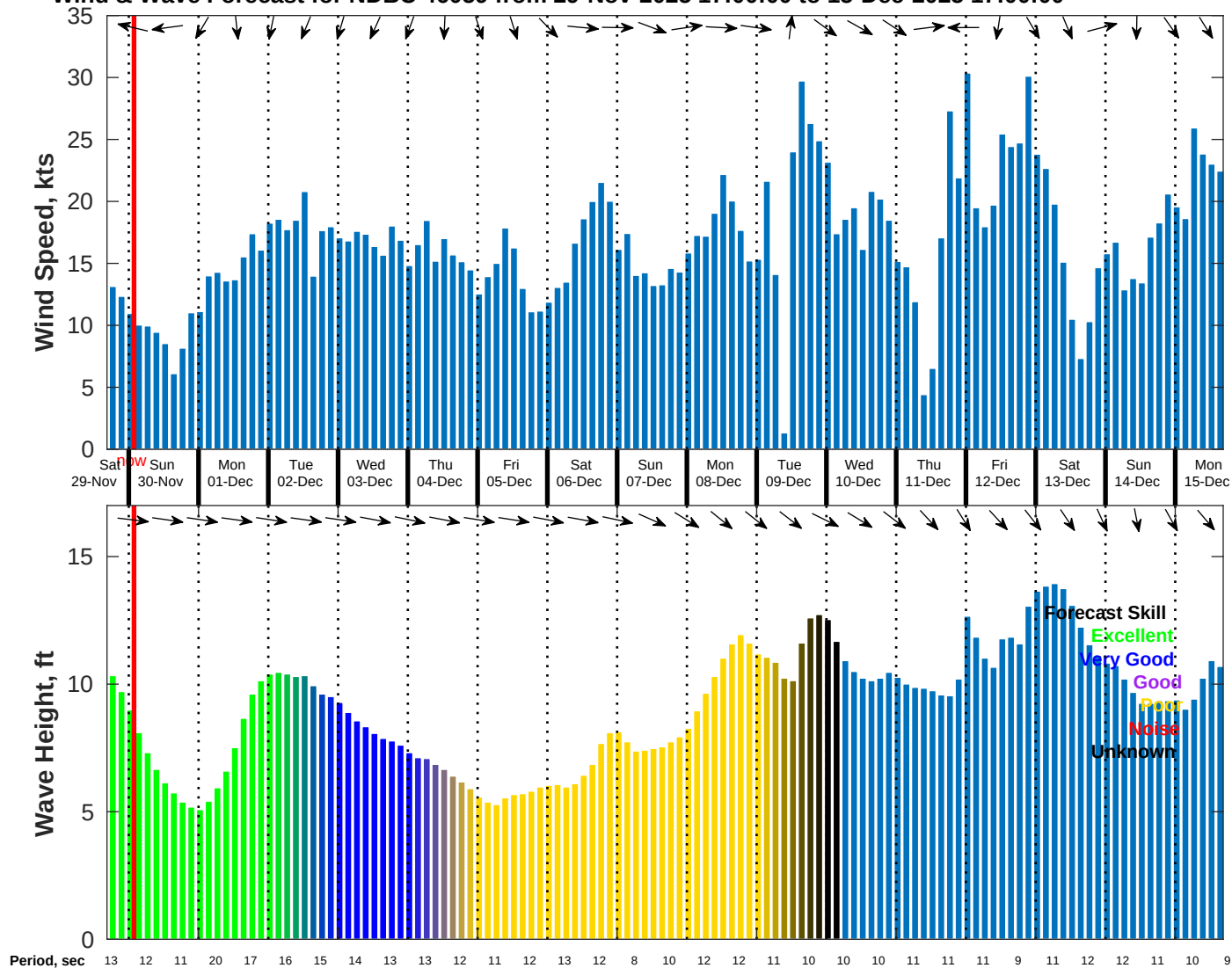
Wind & Wave Forecast for NDBC 46059 from 29-Nov-2025 17:00:00 to 15-Dec-2025 17:00:00
