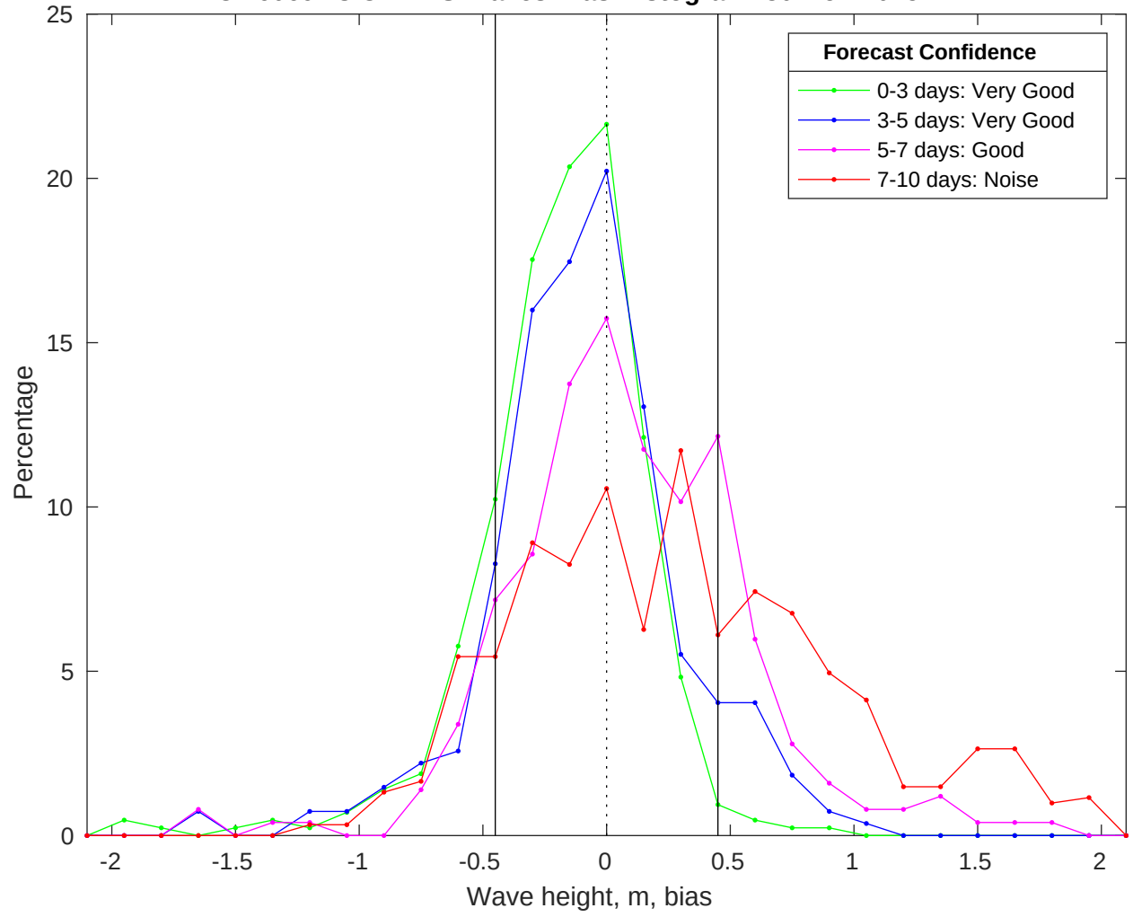
NDBC 46069 vs CMEMS Waves Bias Histogram: 30-Nov-2025
