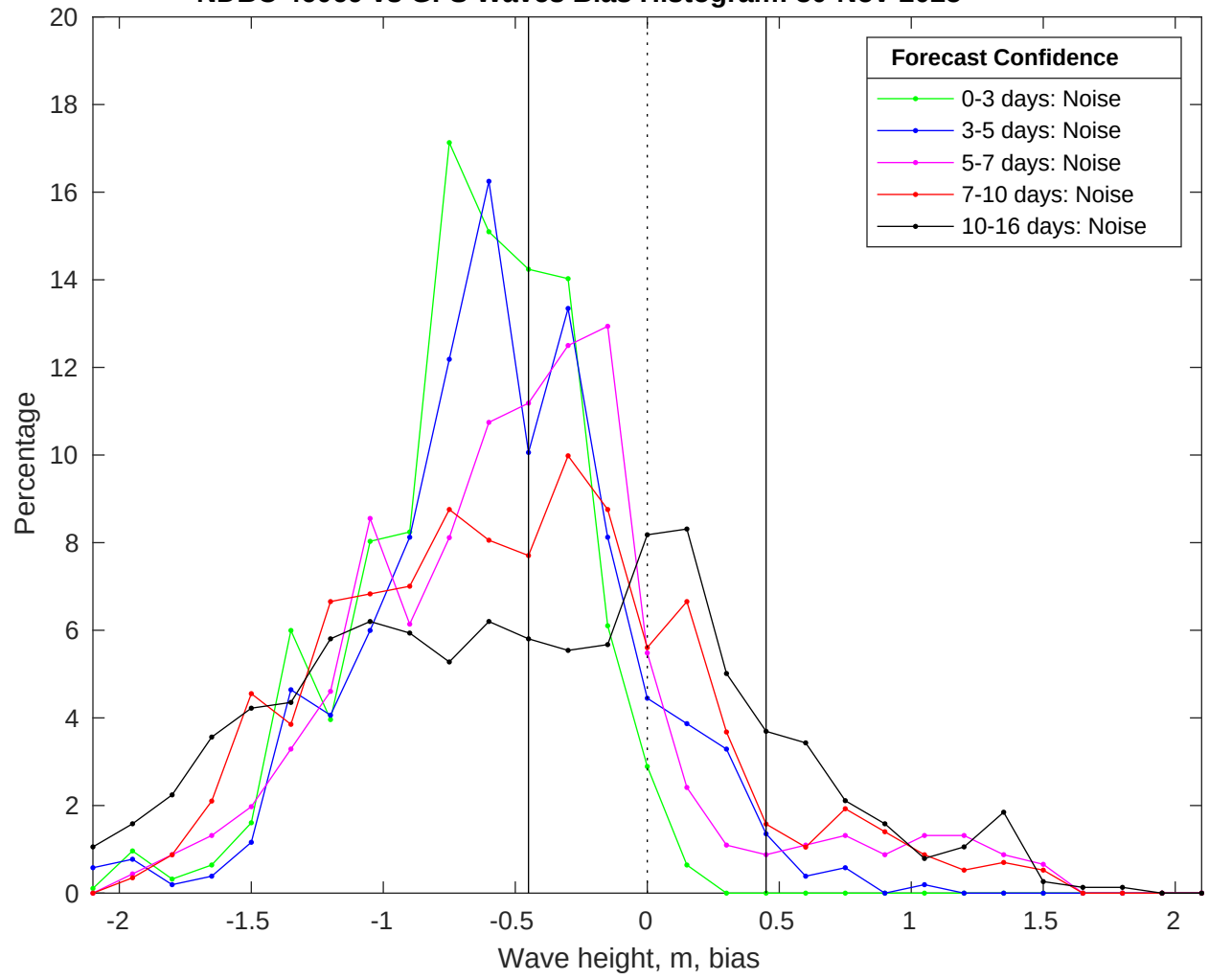
NDBC 46069 vs GFS Waves Bias Histogram: 30-Nov-2025
