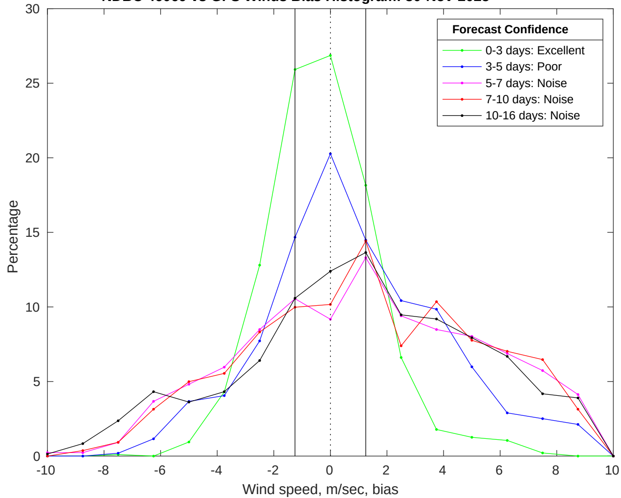
NDBC 46069 vs GFS Winds Bias Histogram: 30-Nov-2025
