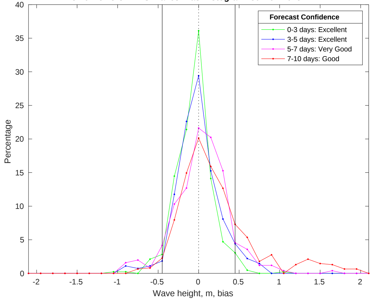
NDBC 46215 vs CMEMS Waves Bias Histogram: 30-Nov-2025
