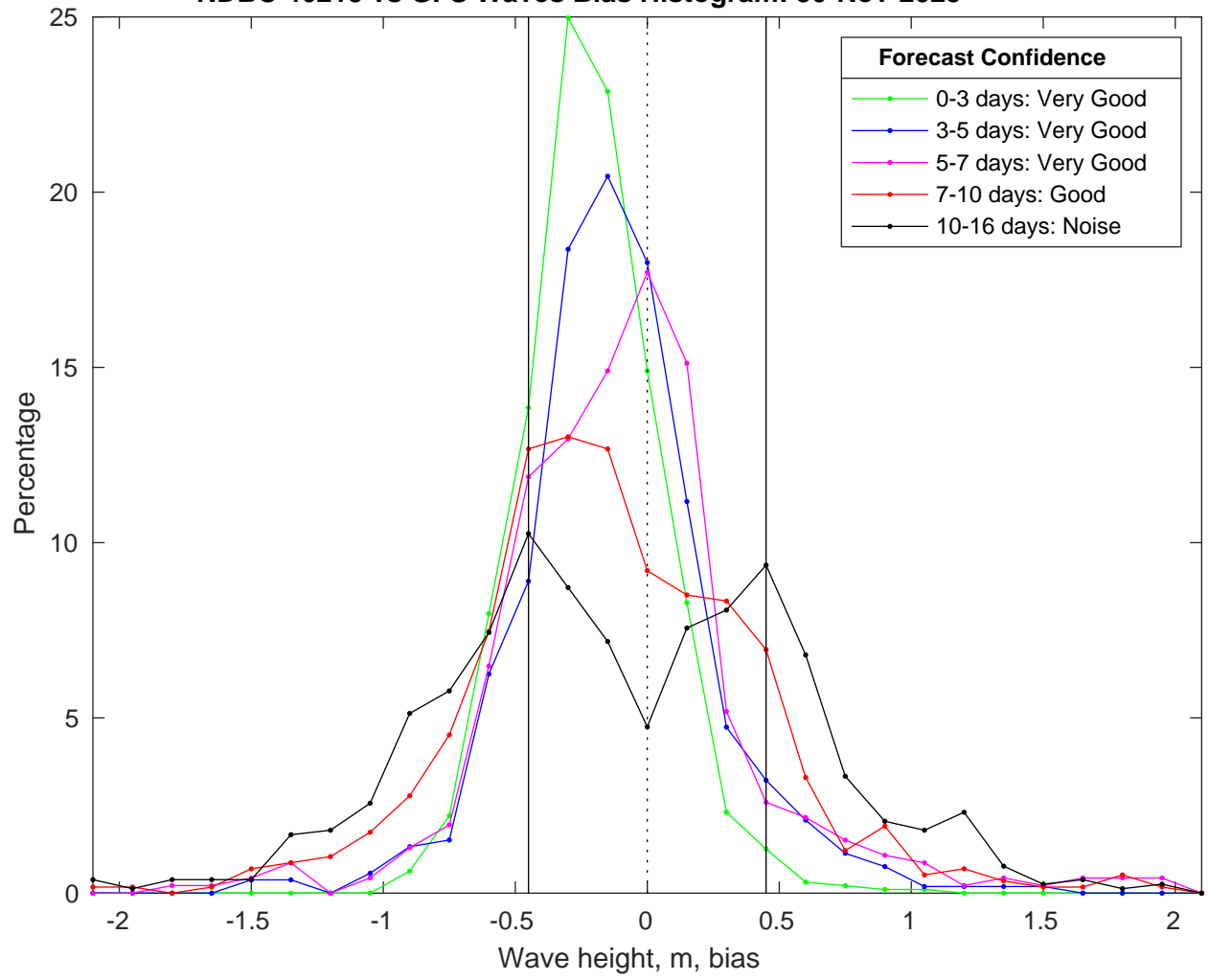
NDBC 46215 vs GFS Waves Bias Histogram: 30-Nov-2025
