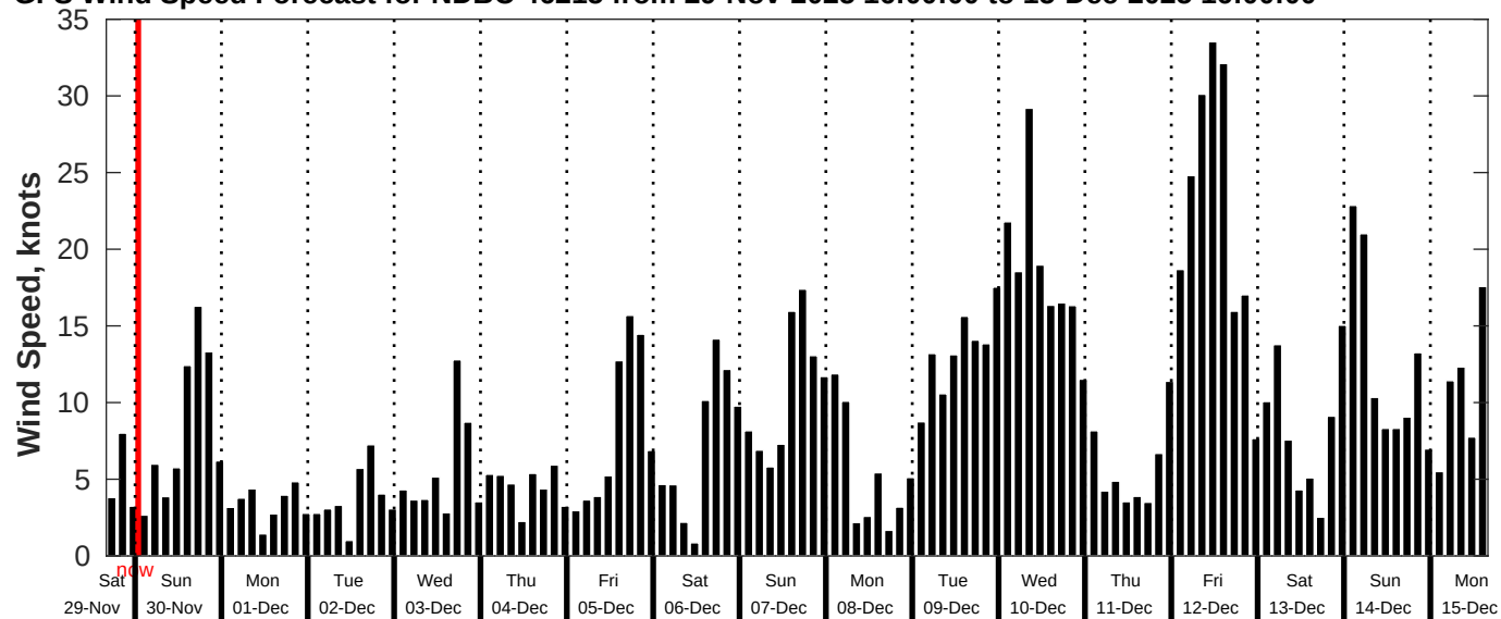
GFS Wind Speed Forecast for NDBC 46215 from 29-Nov-2025 16:00:00 to 15-Dec-2025 16:00:00
