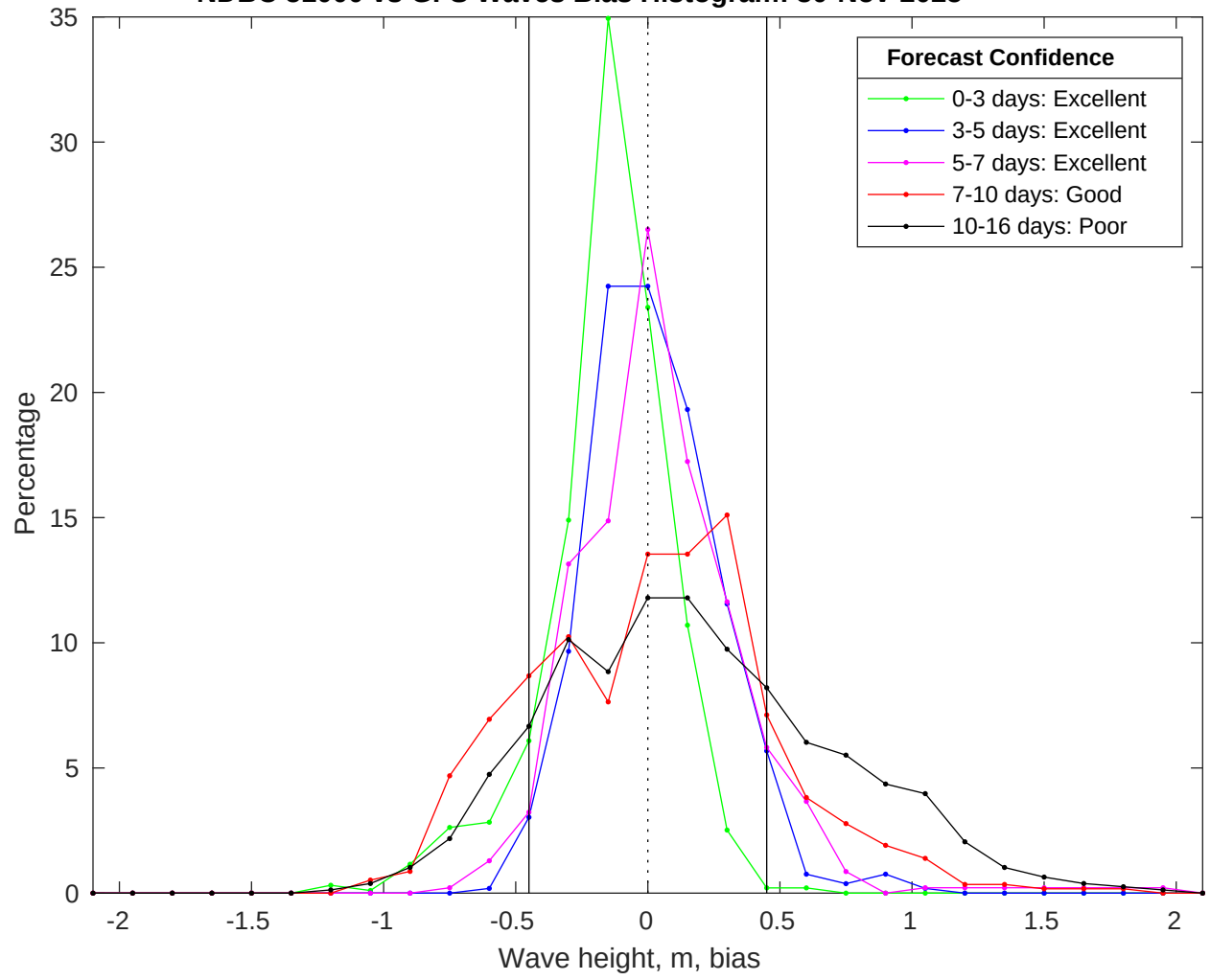
NDBC 51000 vs GFS Waves Bias Histogram: 30-Nov-2025
