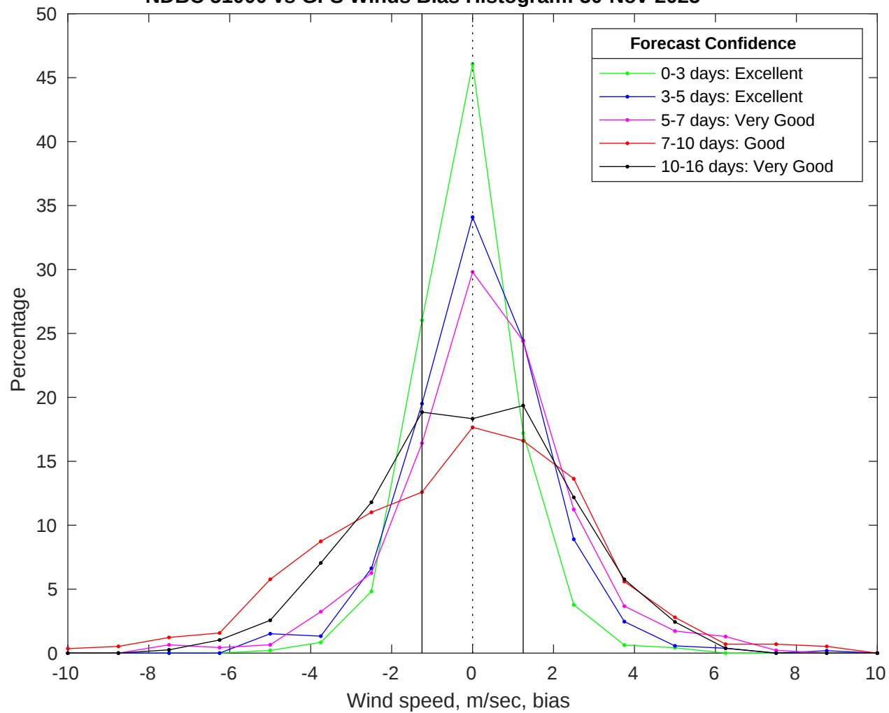
NDBC 51000 vs GFS Winds Bias Histogram: 30-Nov-2025
