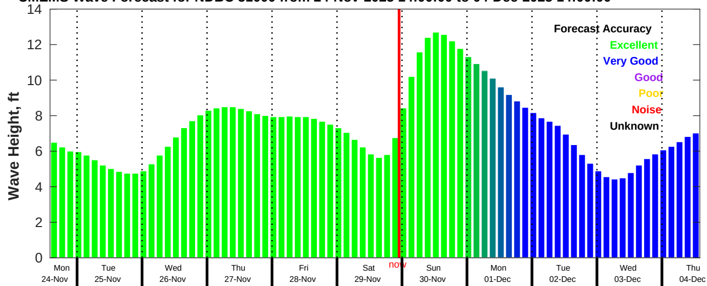
CMEMS Wave Forecast for NDBC 51000 from 24-Nov-2025 14:00:00 to 04-Dec-2025 14:00:00
