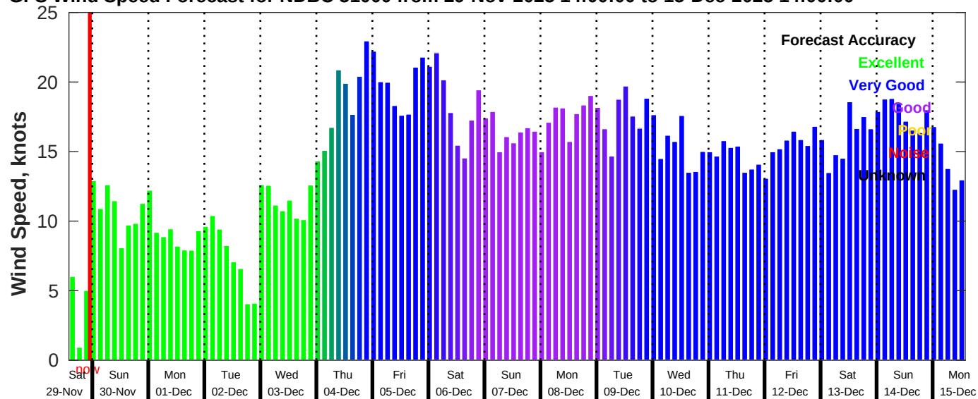
GFS Wind Speed Forecast for NDBC 51000 from 29-Nov-2025 14:00:00 to 15-Dec-2025 14:00:00
