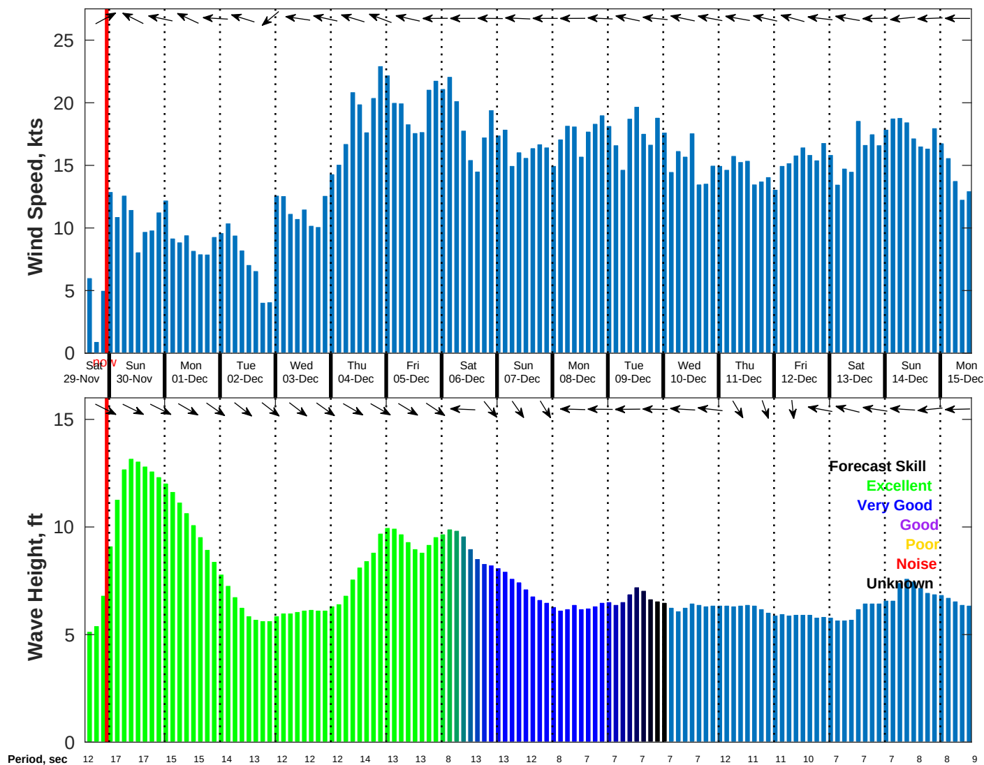
Wind & Wave Forecast for NDBC 51000 from 29-Nov-2025 14:00:00 to 15-Dec-2025 14:00:00
