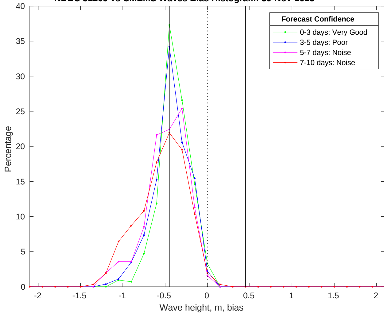
NDBC 51209 vs CMEMS Waves Bias Histogram: 30-Nov-2025
