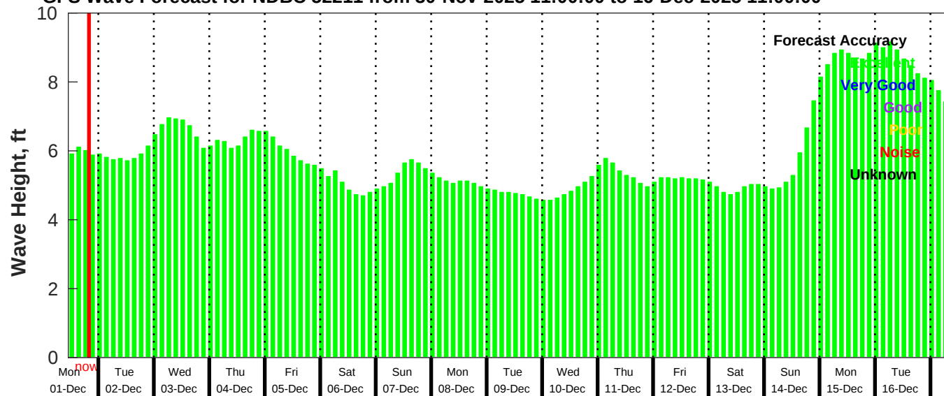
GFS Wave Forecast for NDBC 52211 from 30-Nov-2025 11:00:00 to 16-Dec-2025 11:00:00
