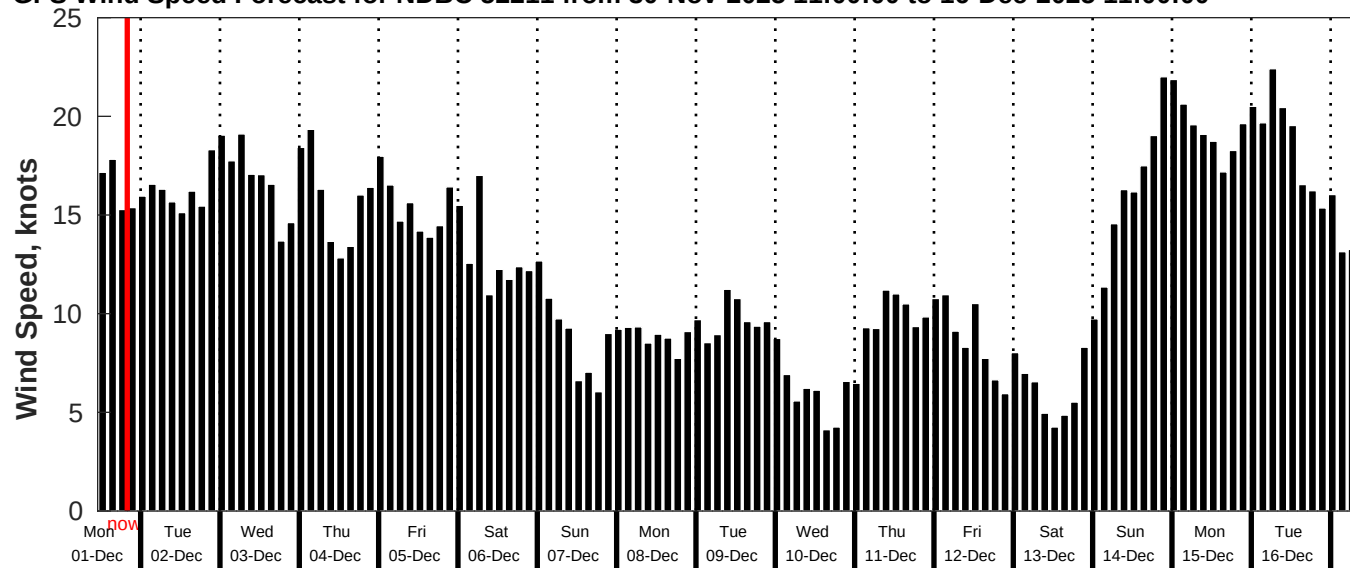
GFS Wind Speed Forecast for NDBC 52211 from 30-Nov-2025 11:00:00 to 16-Dec-2025 11:00:00
