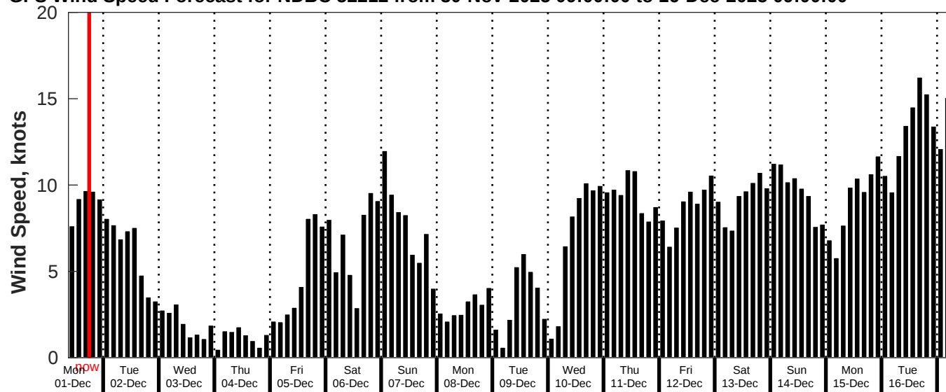
GFS Wind Speed Forecast for NDBC 52212 from 30-Nov-2025 09:00:00 to 16-Dec-2025 09:00:00
