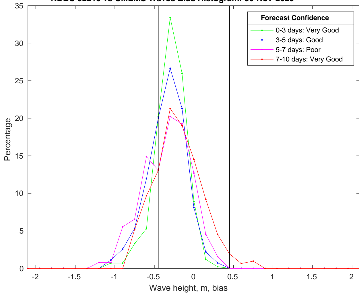
NDBC 52213 vs CMEMS Waves Bias Histogram: 30-Nov-2025
