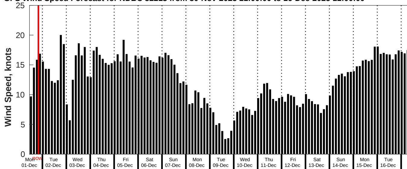
GFS Wind Speed Forecast for NDBC 52213 from 30-Nov-2025 11:00:00 to 16-Dec-2025 11:00:00
