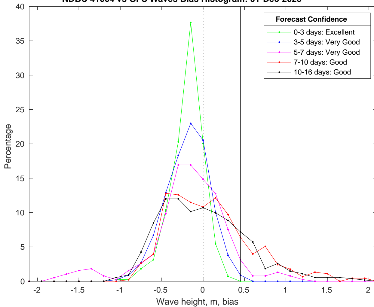
NDBC 41004 vs GFS Waves Bias Histogram: 01-Dec-2025
