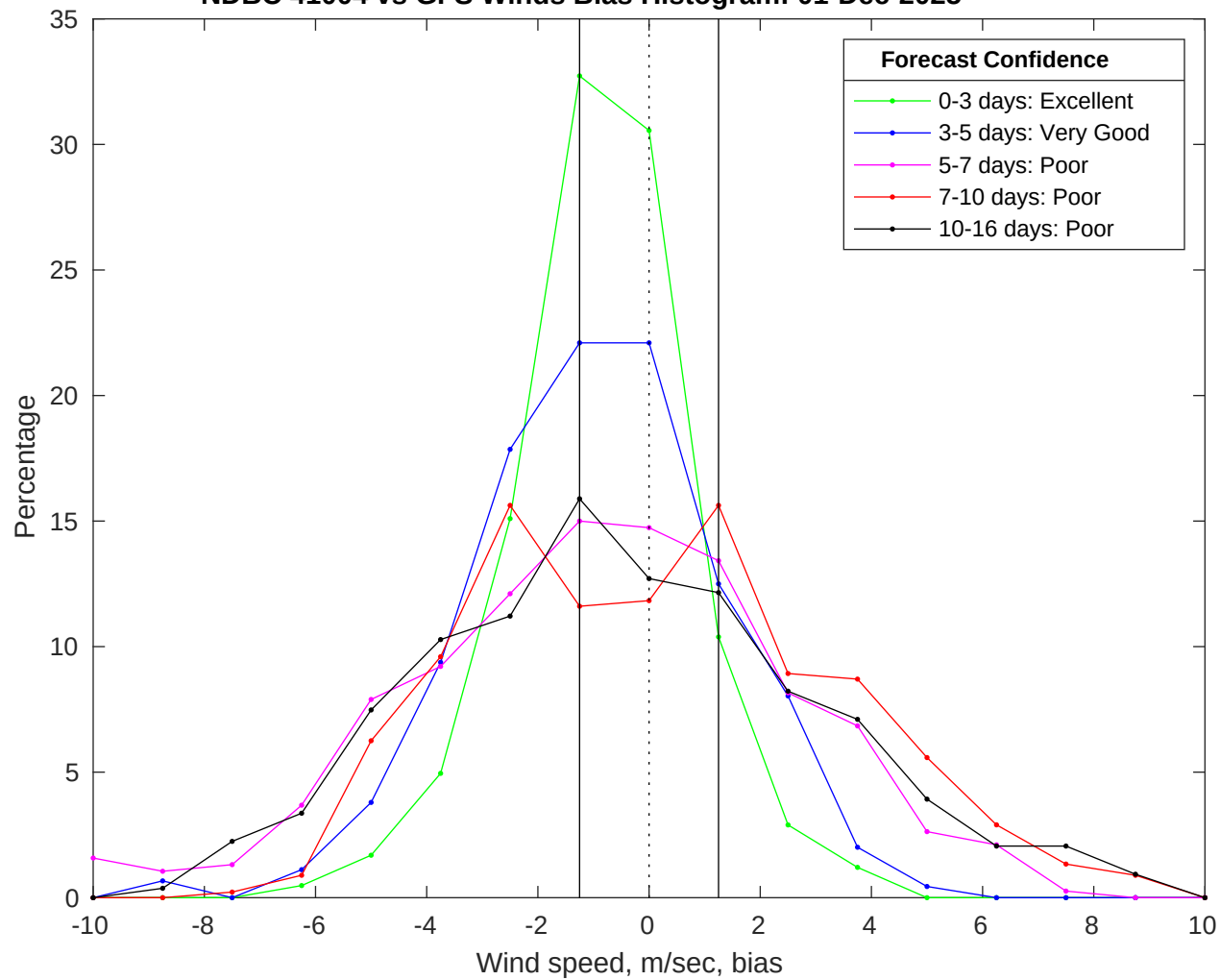
NDBC 41004 vs GFS Winds Bias Histogram: 01-Dec-2025
