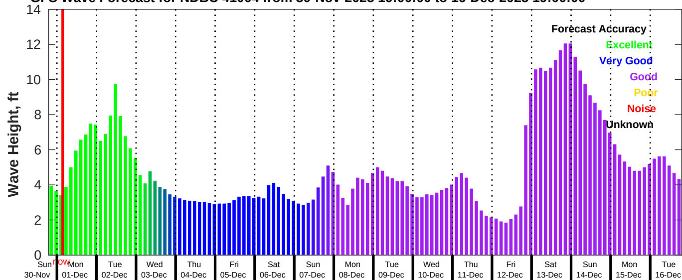
GFS Wave Forecast for NDBC 41004 from 30-Nov-2025 19:00:00 to 16-Dec-2025 19:00:00
