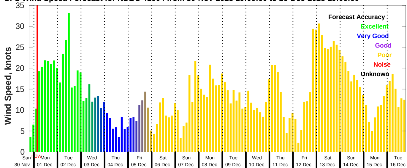
GFS Wind Speed Forecast for NDBC 41004 from 30-Nov-2025 19:00:00 to 16-Dec-2025 19:00:00
