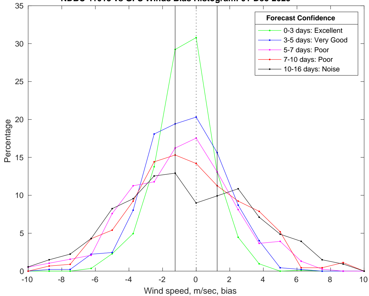
NDBC 41013 vs GFS Winds Bias Histogram: 01-Dec-2025
