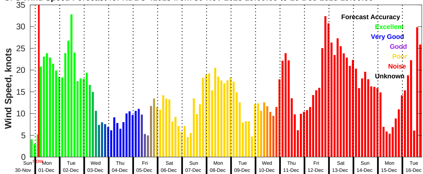
GFS Wind Speed Forecast for NDBC 41013 from 30-Nov-2025 19:00:00 to 16-Dec-2025 19:00:00
