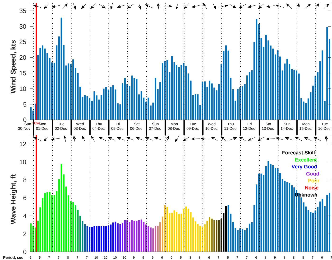
Wind & Wave Forecast for NDBC 41013 from 30-Nov-2025 19:00:00 to 16-Dec-2025 19:00:00
