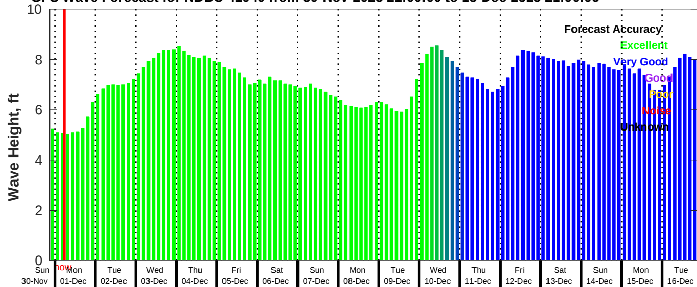
GFS Wave Forecast for NDBC 41040 from 30-Nov-2025 21:00:00 to 16-Dec-2025 21:00:00
