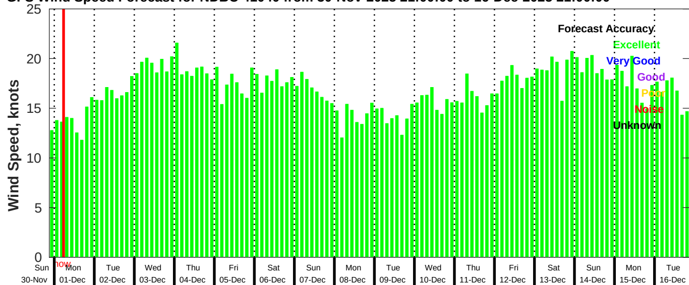
GFS Wind Speed Forecast for NDBC 41040 from 30-Nov-2025 21:00:00 to 16-Dec-2025 21:00:00
