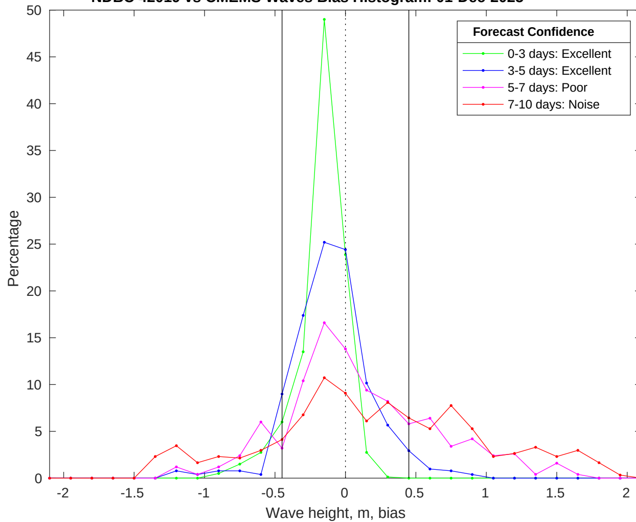
NDBC 42019 vs CMEMS Waves Bias Histogram: 01-Dec-2025
