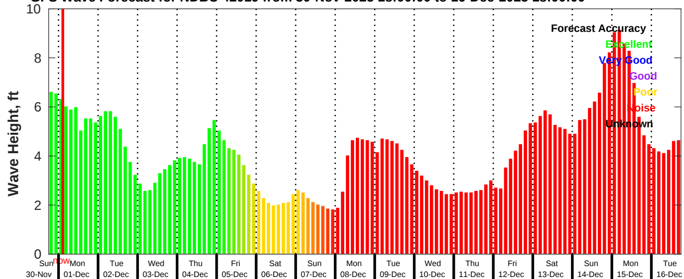
GFS Wave Forecast for NDBC 42019 from 30-Nov-2025 18:00:00 to 16-Dec-2025 18:00:00
