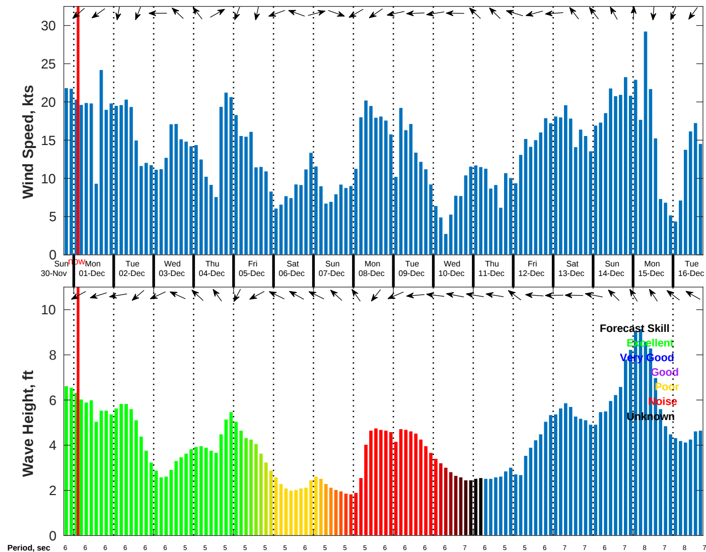
Wind & Wave Forecast for NDBC 42019 from 30-Nov-2025 18:00:00 to 16-Dec-2025 18:00:00
