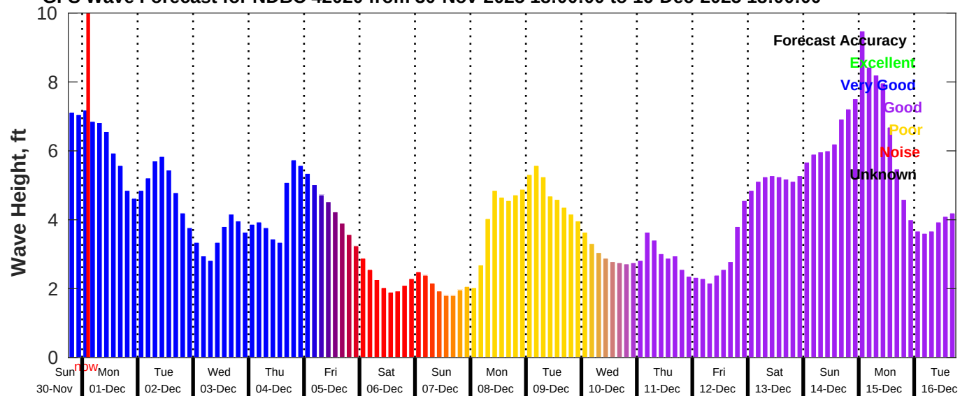
GFS Wave Forecast for NDBC 42020 from 30-Nov-2025 18:00:00 to 16-Dec-2025 18:00:00
